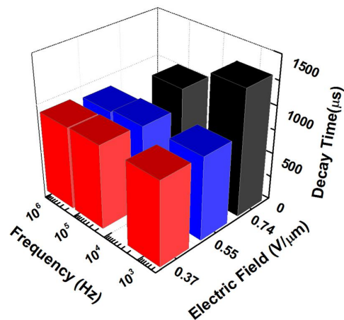
FIG. 6. The decay time of the PS-BPLCs with different electric fields during polymerization of 0.37 V/ \mu\text{m} , 0.55 V/ \mu\text{m} , and 0.74 V/ \mu\text{m} .
