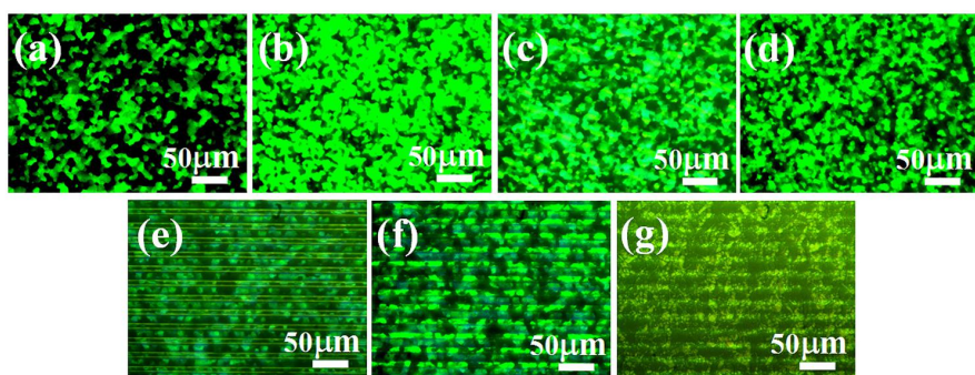
FIG. 1. Texture of BPLC after polymer stabilization with different electric fields: (a) 0 \text{ V}/\mu\text{m} , (b) 0.18 \text{ V}/\mu\text{m} , (c) 0.37 \text{ V}/\mu\text{m} , (d) 0.55 \text{ V}/\mu\text{m} , (e) 0.74 \text{ V}/\mu\text{m} , (f) 0.92 \text{ V}/\mu\text{m} , and (g) 1.1 \text{ V}/\mu\text{m} .
