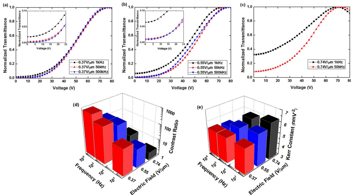
FIG. 4. Normalized V-T curves with electric fields during polymerization at different frequencies of (a) 0.37 \text{ V}/\mu\text{m} , (b) 0.55 \text{ V}/\mu\text{m} , and (c) 0.74 \text{ V}/\mu\text{m} . (d) The contrast ratio and (e) the Kerr constant of the PS-BPLCs with different electric fields during polymerization of 0.37 \text{ V}/\mu\text{m} , 0.55 \text{ V}/\mu\text{m} , and 0.74 \text{ V}/\mu\text{m} .
