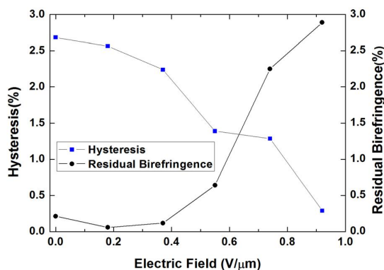
FIG. 5. The hysteresis and residual birefringence of PS-BPLCs with different electric fields during polymerization.
